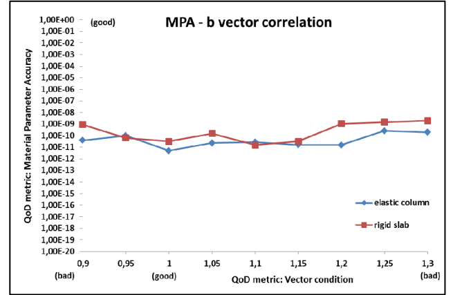
Figure 5: Results of elastic column (EC) and rigid slab (RS) relating to the material parameter accuracy (MPA) and the vector condition (VC) of vector b
