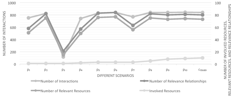
Figure 3. Relevant resources found and their relation with involved resources and interactions
