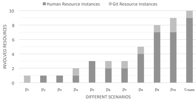
Figure 2. Scenarios used in the application
