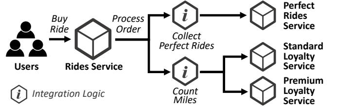
Fig. 1. Example microservice architecture with service integration points.
