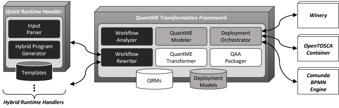
Figure 3: System architecture of the extended MODULO framework
